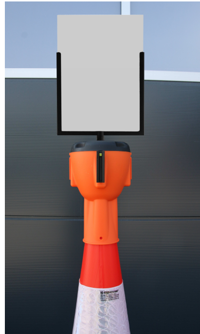
Pict. 2: ALCT-SH = (signholder, DIN A4) on cone topper ALCT-O (cone and cone-topper not included)
